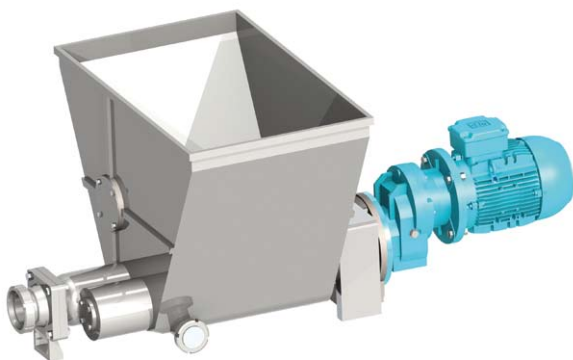
BLADE FEEDER WITH 2 PRE-FEEDING SCREWS
