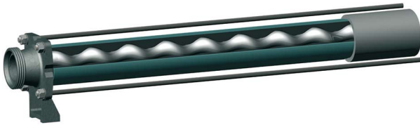
4 stages - max. 24 bar
