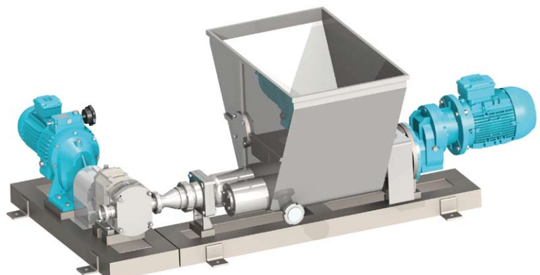
BLADE FEEDER WITH LOBE PUMP
